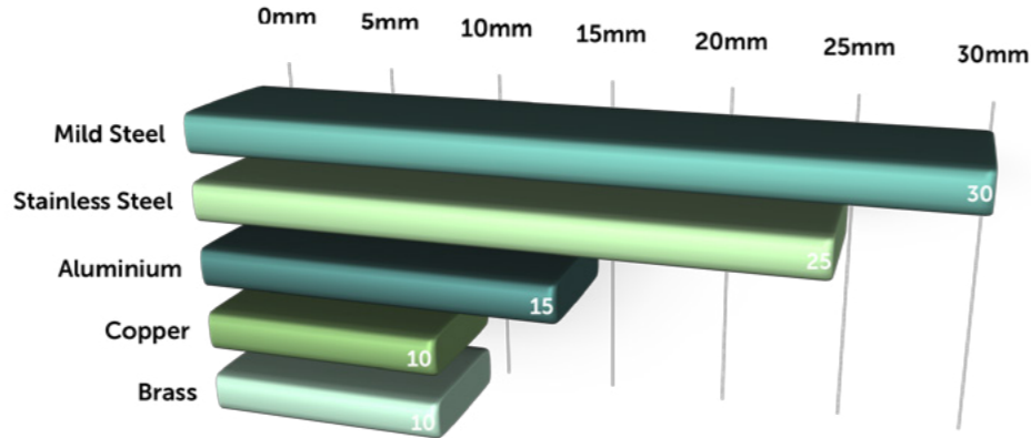
Maximum Sheet Thickness Cut
